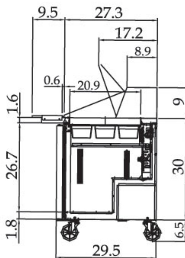
SIDE VIEW
