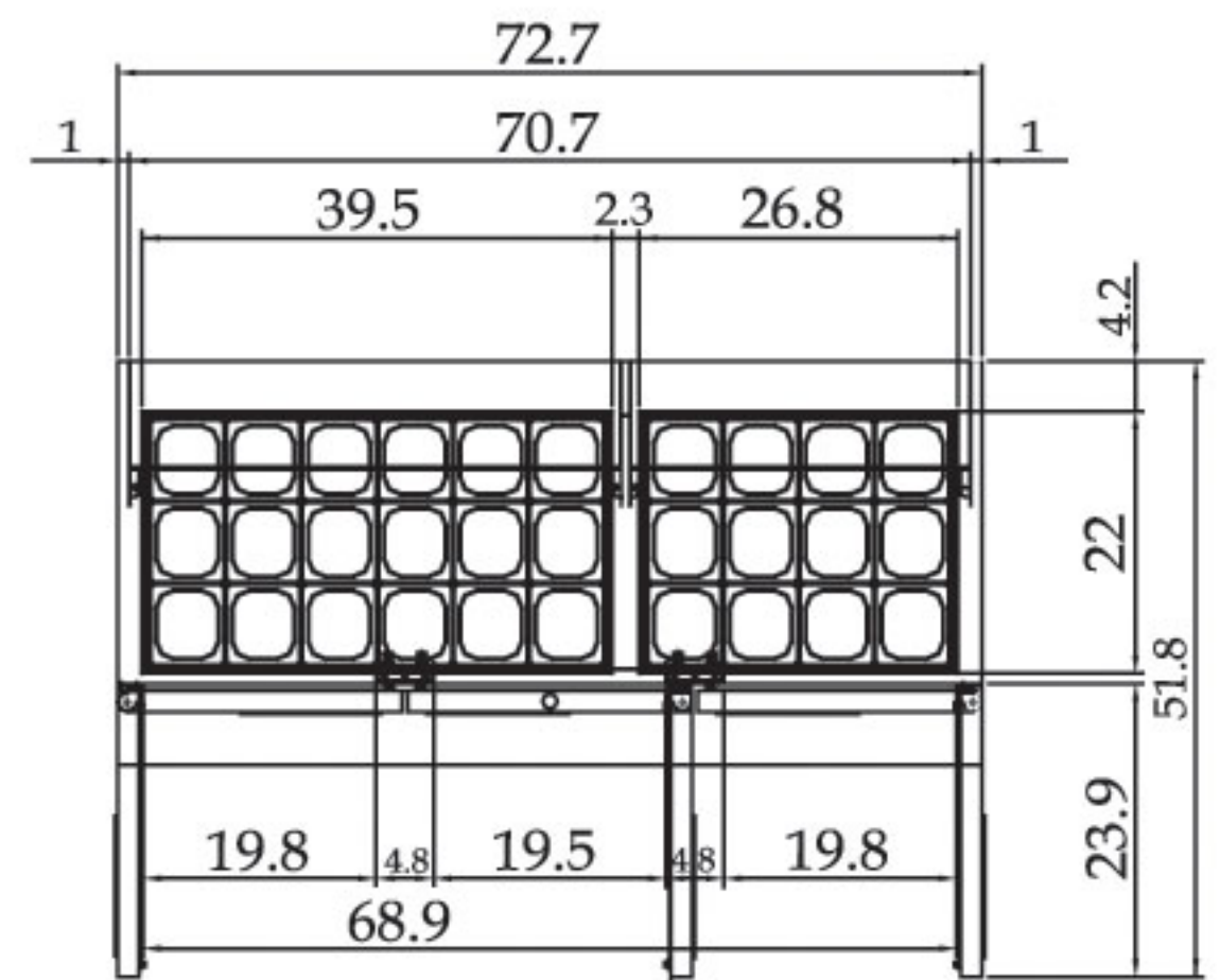
TST-72SD-30 PLAN VIEW
