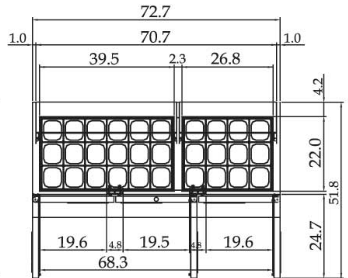
TST-72SD-30 PLAN VIEW
