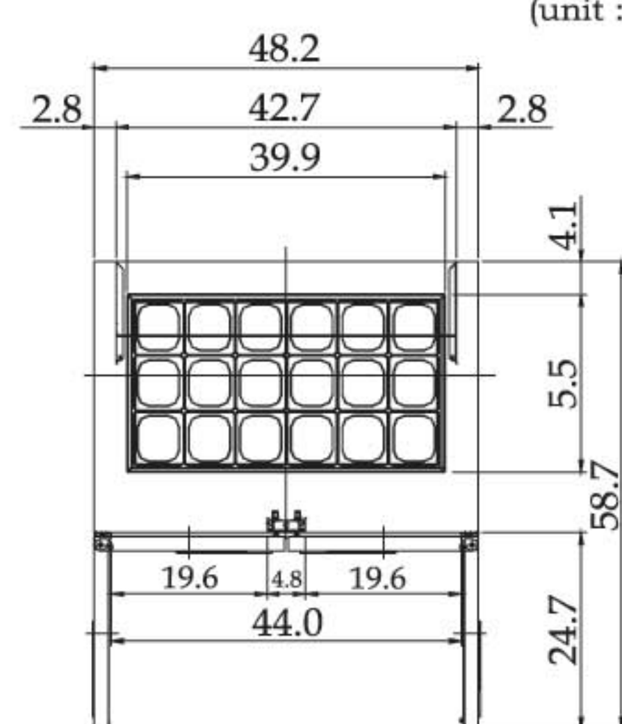
TST-48SD-18 PLAN VIEW
