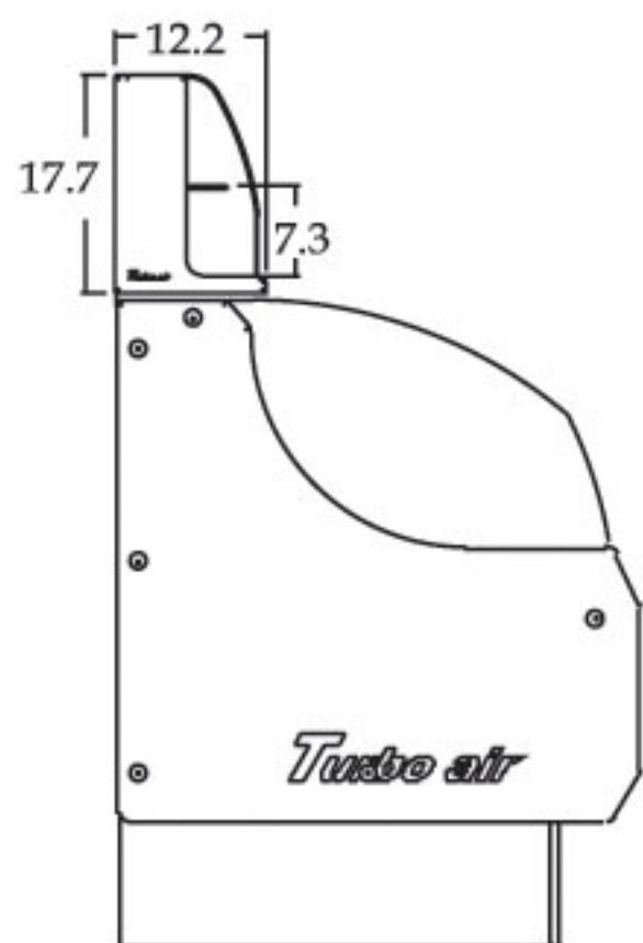
TOM-S COMBINATION WITH TOMD-H SIDE VIEW
